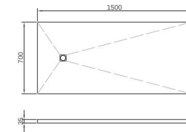
T103 Size: 1500x700x35mm
