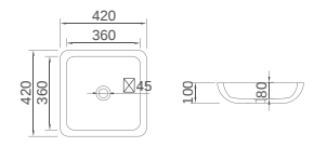
K-1320 Size: 420x420x100mm
