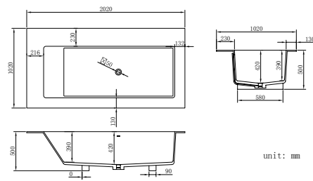
B069 Size: 2020x1020x500mm
