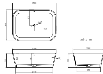
B071 Size: 1700x1200x550mm
