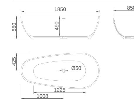
B001-B Size: 1850x850x550mm
