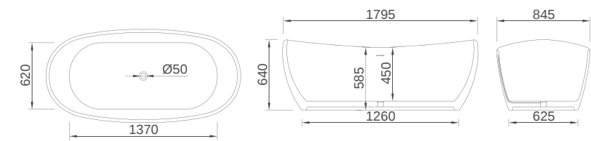
B034 Size: 1795x845x640mm
