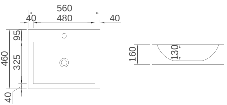
K-0612B Size: 560x460x160mm
