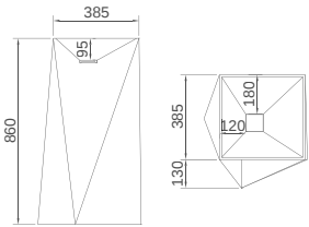
R-1387 Size: 385x385x860mm
