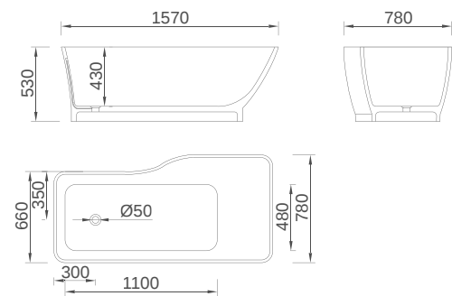
B005 Size: 1570x780x530mm
