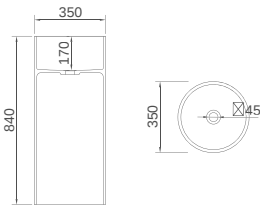
R-1389 Size: Dia350x840mm
