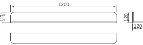
A1560-2 Size: 1200X120X120mm
