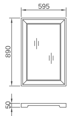
A1579 Size: 890x595x50mm
