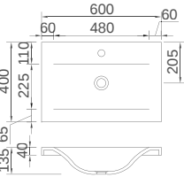
K-1250 Size: 600x400x135mm
