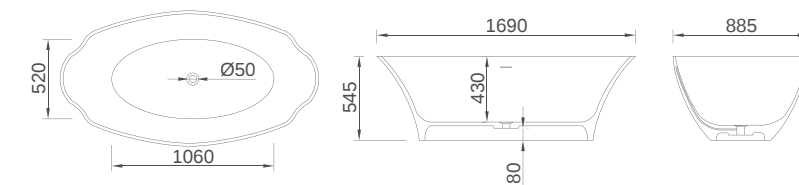
B011 Size: 1690x885x545mm
