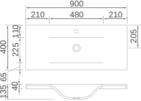
K-1252 Size: 900x400x135mm
