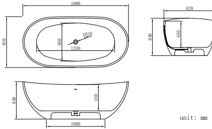
B054 Size: 1800x870x640mm
