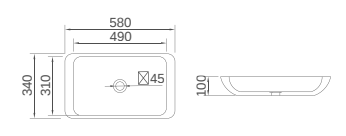
K-1321 Size: 580x340x100mm
