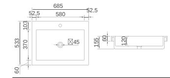
K-1345 Size: 685x533x155mm
