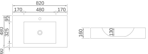
K-0804 Size: 820x480x160mm
