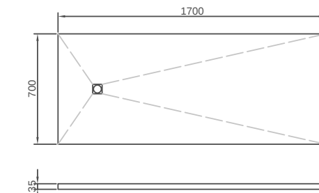
T107 Size: 1700x700x35mm
