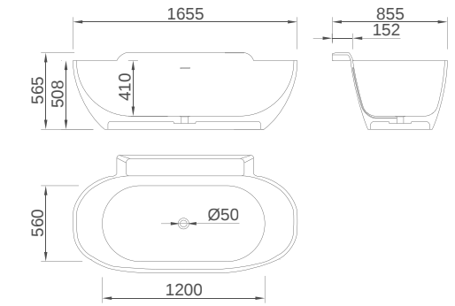
B025 Size: 1655x855x565mm
