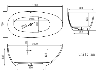
B068 Size: 1600x760x525mm
