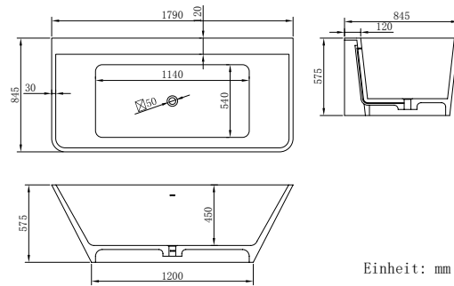
B053 Size: 1790x845x575mm
