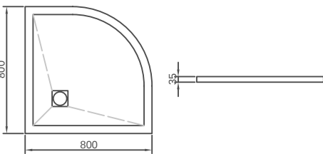
T116 Size: 800x800x35mm
