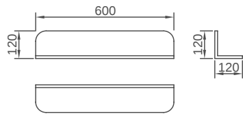
A1560 Size: 600X120X120mm
