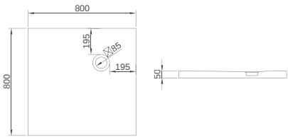
T005 Size: 800x800x50mm
