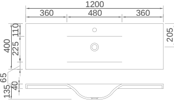
K-1253 Size: 1200x400x135mm
