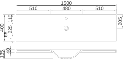
K-1254 Size: 1500x400x135mm
