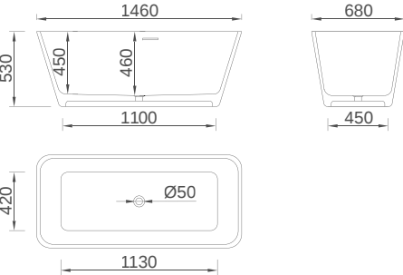
B043 Size: 1460x680x530mm
