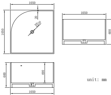
B067 Size: 1050x1050x600mm
