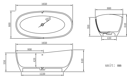
B063 Size: 1650x800x640mm
