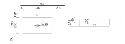
K-1346 Size: 990x533x175mm
