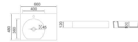
K-1343 Size: 660x480x120mm
