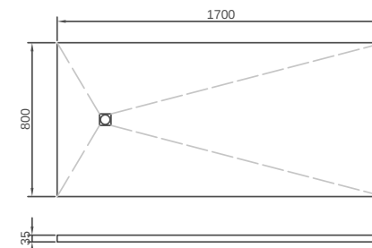
T106 Size: 1700x800x35mm
