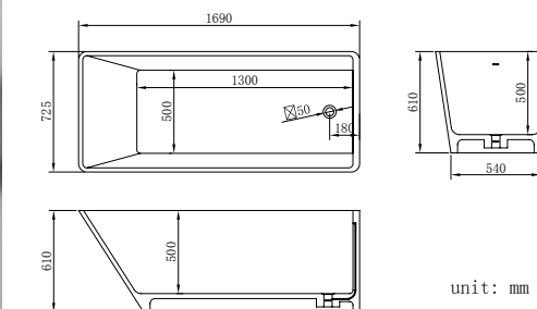
B058 Size: 1690x725x610mm
