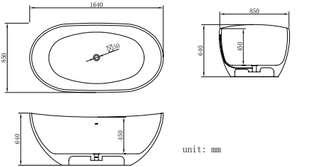
B054-A Size: 1640x850x640mm
