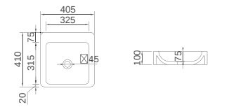
K-1323 Size: 405x410x100mm
