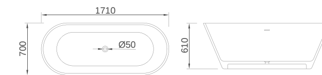
B050 Size: 1710x700x610mm
