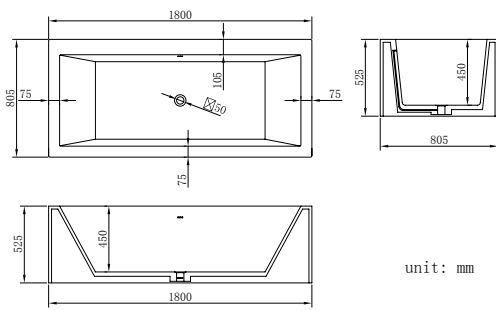
B060 Size: 1800x805x525mm
