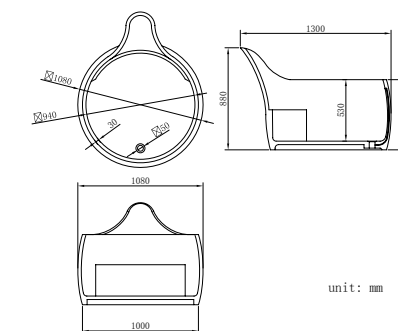
B070 Size: 1300x1080x880mm
