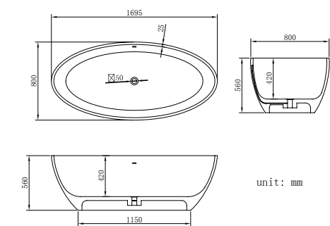
B066 Size: 1695x800x560mm
