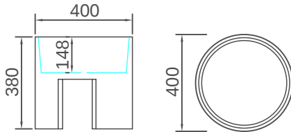
Stool -C Size: Dia400x380mm
