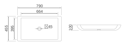
K-1322 Size: 790x455x100mm
