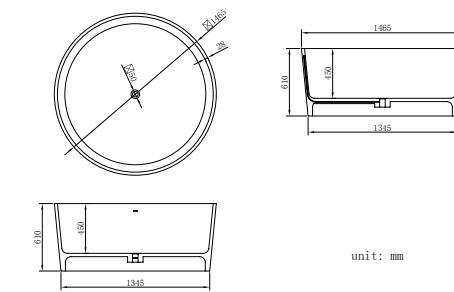
B064 Size: 1465x1465x610mm
