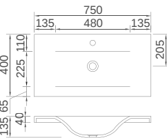
K-1251 Size: 750x400x135mm
