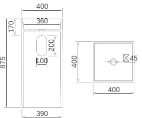
R-1382 Size: 400x400x875mm
