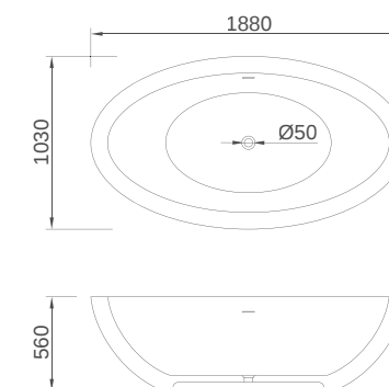
B048 Size: 1880x1030x560mm
