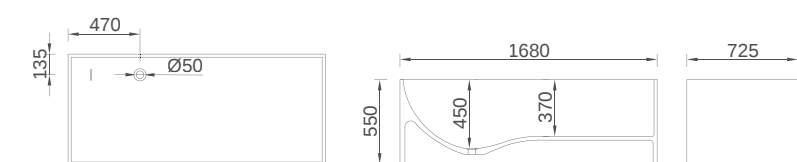
B029 Size: 1680x725x550mm
