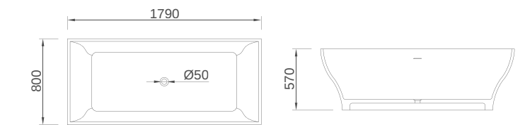
B052 Size: 1790x800x570mm
