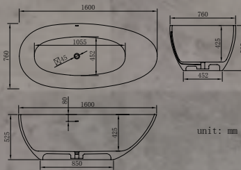
B068-A Size: 1600x760x525mm
